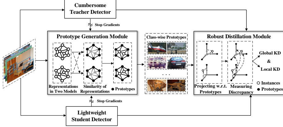
Fig. 2. The proposed framework for distilling object detectors with global knowledge. A prototype generation module (PGM) is first deployed to find the prototypes for each class based on the similarity of their representations in TS -space. A robust distillation module (RDM) is then designed to construct reliable global knowledge w.r.t. the prototypes and measure their discrepancy for robust knowledge distillation.
