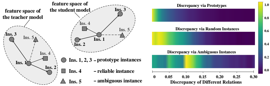
Fig. 1. Left: the prototypes are representative and play roles as a common group of basis vectors in TS -space. Although the absolute roles of Ins. 4 is different in TS -space, its representations, e.g., the relations, w.r.t. prototypes are similar while Ins. 5 shows the representation of much dissimilar. Right: on COCO dataset [28] with Faster-RCNN detector [36], we show the discrepancy of relations between instances and three types of basis in TS -space. 10 instances are selected for each class as the bases and others are used for measuring the discrepancy of relations in TS -space. The relations with prototypes show much smaller discrepancy than others.
